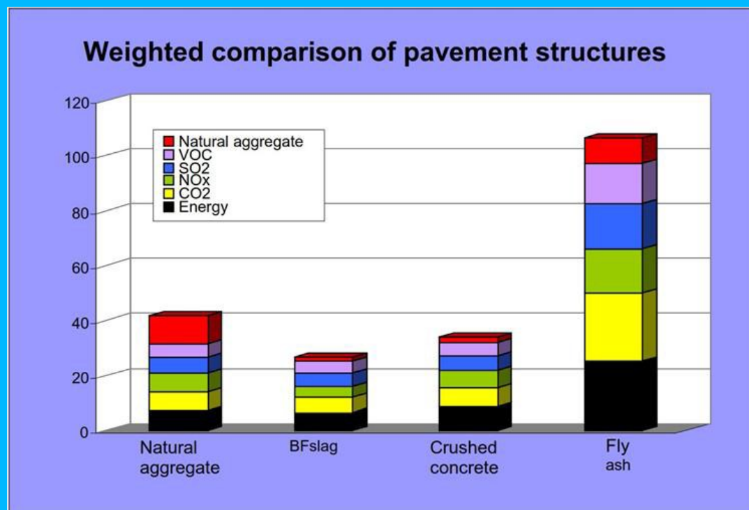
Figure 4.4 Results from Meli calculations
