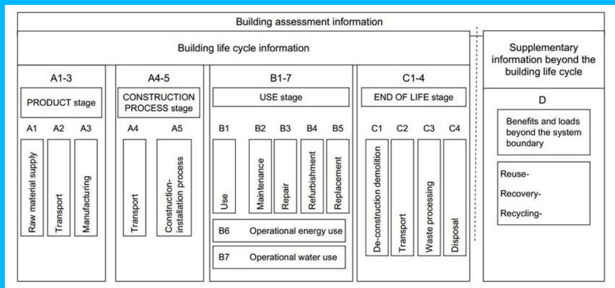
Figure 4.1. LCA stages according to EN 15978:2011.
